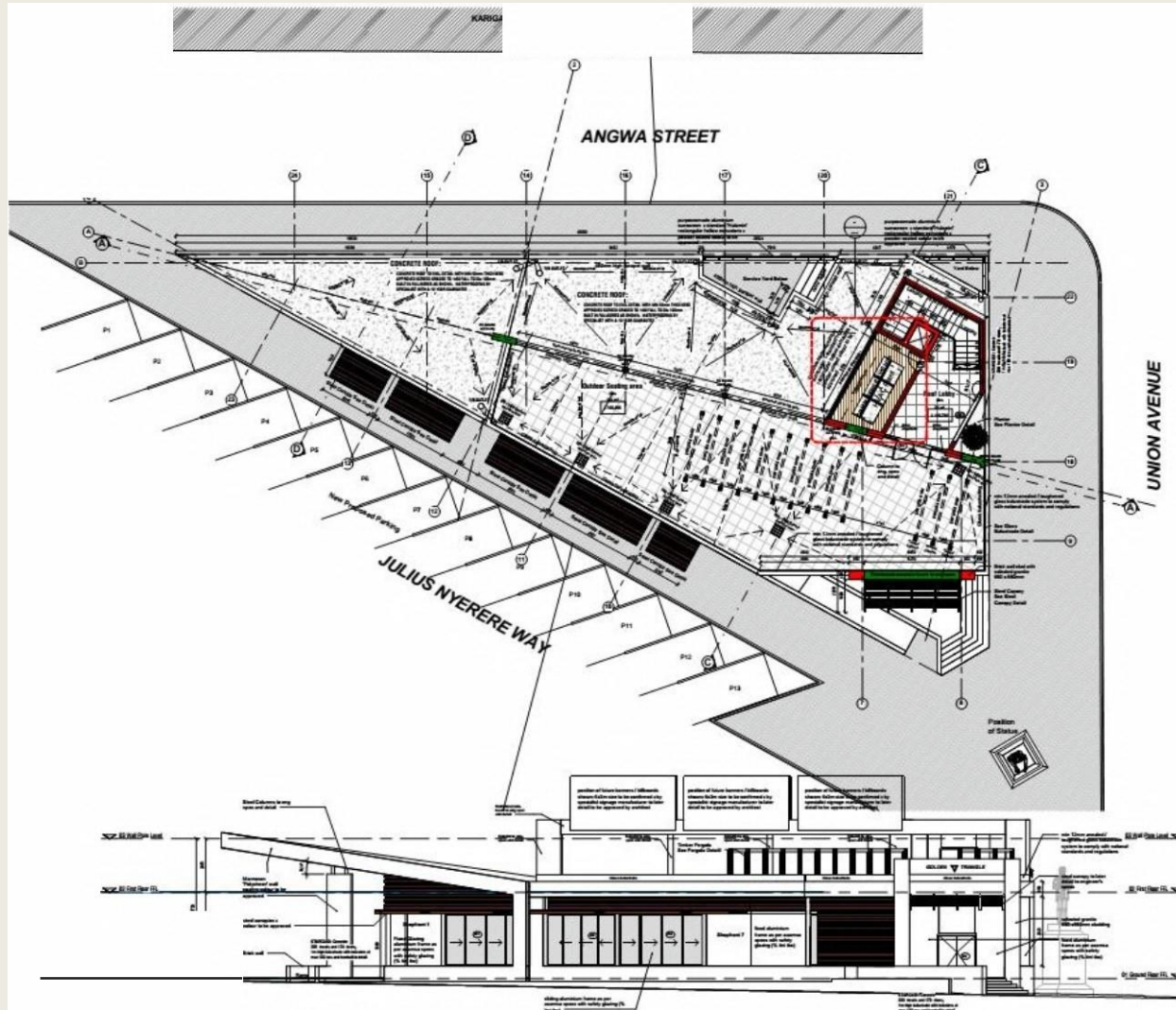
FIRST FLOOR LAYOUT
